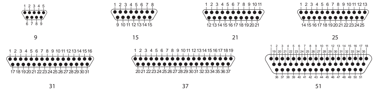
Mating face of pin connector. Socket connector contact numbers are reversed.
