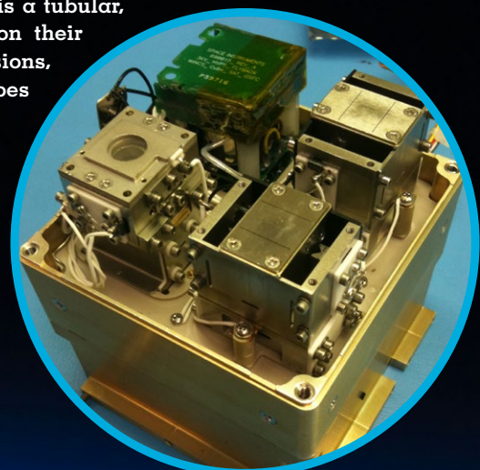
Close-up of the Winds-Ion-Neutral Composition Suite (WINDS) instrument: four spectrometers and three detectors in a three-inch, 1.3 watt package—specially designed to fly on Cubesats.
