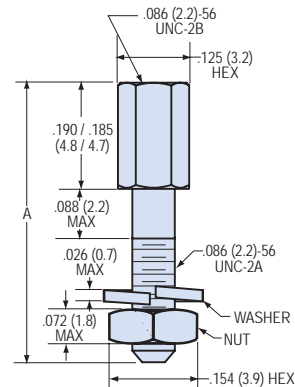
Figure 1 #2-56 Jackpost
