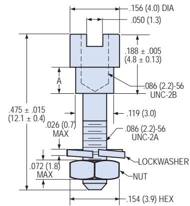
Figure 1 #2-56 Jackpost
