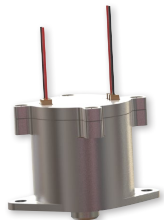
1/4 inch unit with 5,000 pound preload and conventional wire lead interface
