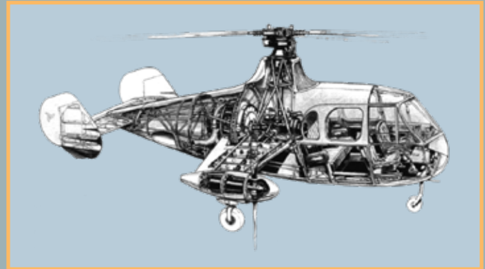
Schematic drawing of a prototype Fairey Gyrodyne rotorcraft from 1946
