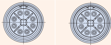
Mating Face of Pin Contacts Mating Face of Socket Contacts
