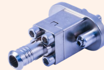
-06 plug, with retaining plate for EMI shield termination and strain relief of ribbon or round fiber cable
