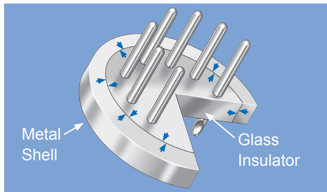
In Matched Seal hermetics, thermal expansion of the glass and metal materials are nearly the same. The stress in the glass is therefore relatively small—an important factor in the design of Micro-D hermetic connectors, due to varying degrees of stress on the glass caused by the rectangular shape.
