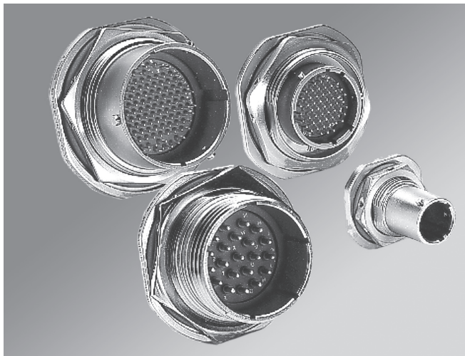
In hermetic connector manufacturing, the glass material is introduced either as separate glass beads or as a pre-formed glass seal insulator tooled to precise dimensions. The glass must be exactly selected for each application according to its ability to form a strong bond with the metal materials.
