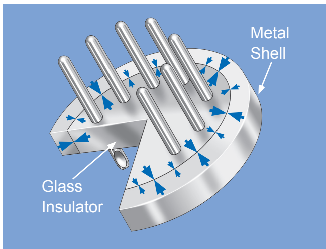
In Mismatched (Compression) Seals, the thermal expansion/contraction of the metal exceeds that of the glass. During cooling, the metal contracts into the already solidifying glass to form an extremely robust compression bond.
