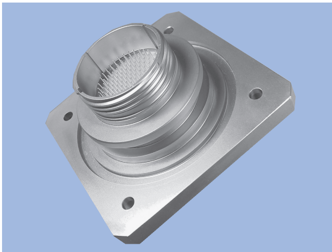
Glenair typically specifies stainless steel, titanium or Kovar for its hermetic products to provide an effective barrier against gas ingress and corrosion caused by dew point condensation. The hermetic sealing helps insure against damage to sensitive electronic systems and components.
