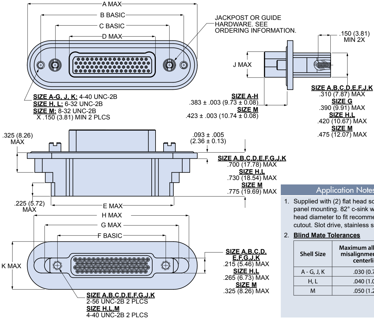
791-020S Dimensions
