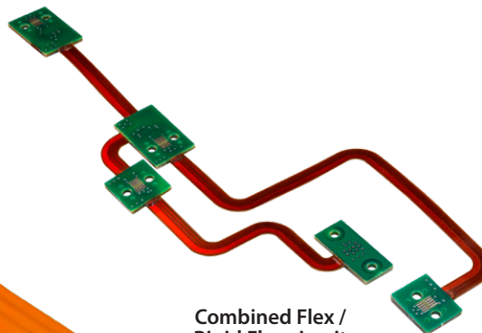
High-shock matched-impedance Thermo assembly with flex circuit
