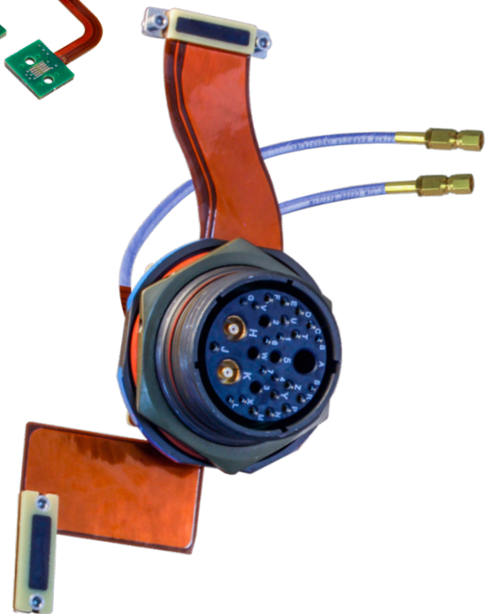
Hybrid flex/rigid flex multibranch Micro-D and Series 23 SuperNine flex assembly with discrete RF circuits
